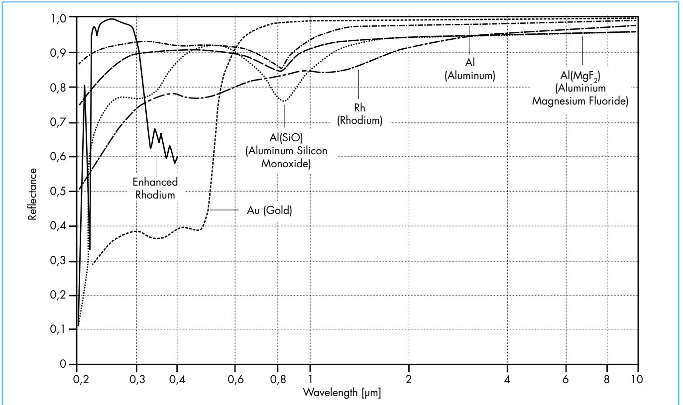
Typical near normal incidence reflectance of different coatings
