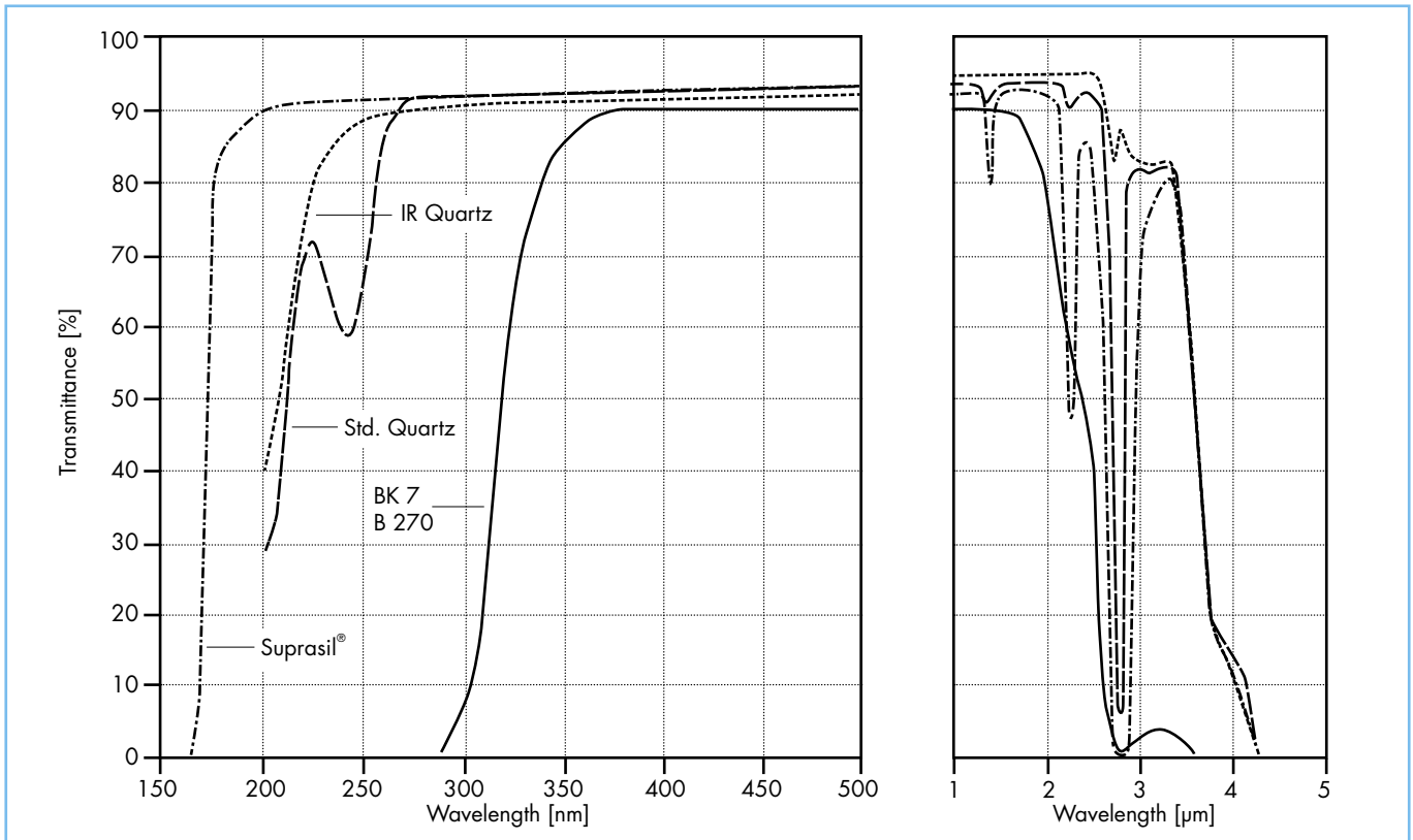
Transmittance of 10 mm thick quartz and glass windows
