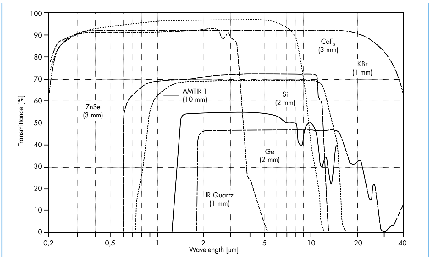
Transmittance of UV and IR materials
