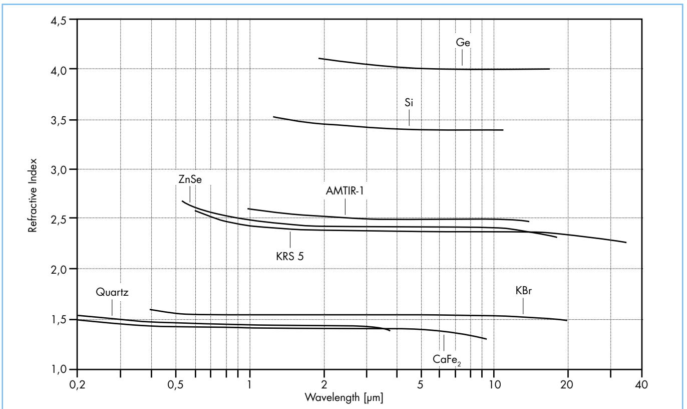
Refractive index of optical materials
