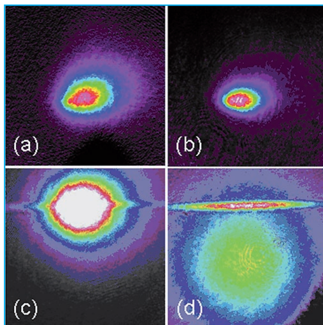
Fig. 2 Absorption images of the atoms (a) in the magneto-optical trap (MOT), (b) in the dark MOT, (c) in the optical trap surrounded by the untrapped atoms, and (d) in the optical trap with untrapped atoms falling under the gravity.
